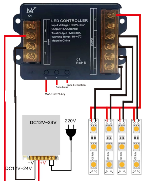
Wiring diagram
