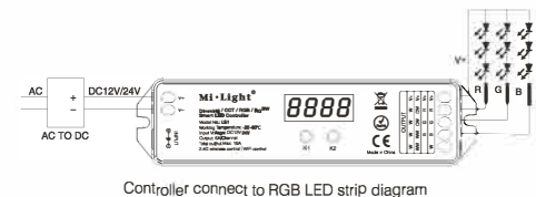
Controller connect to RGB LED strip diagram
