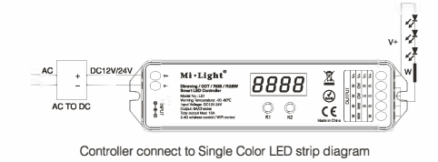
Controller connect to Single Color LED strip diagram
