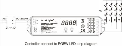
Controller connect to RGBW LED strip diagram
