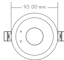
Ceiling (drill hole \varnothing 86mm)
