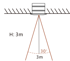
Ceiling mounting pattern
