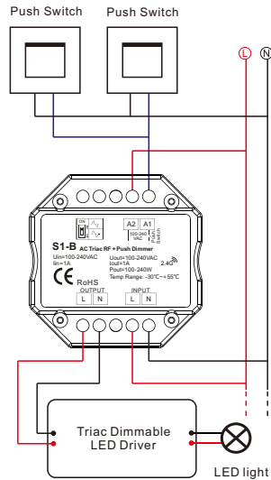
S1-B connect with dimmable LED driver
