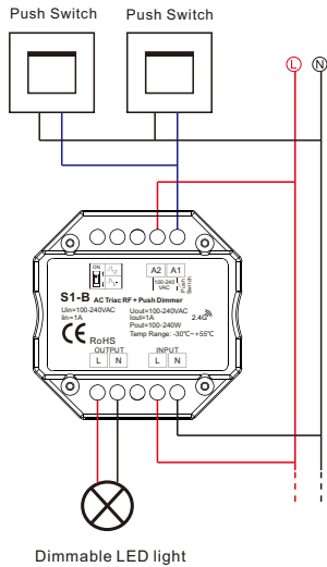
S1-B connect with dimmable LED light
