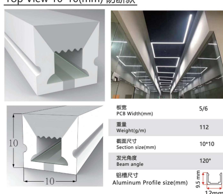
Top View 10*10(mm) 防断款
