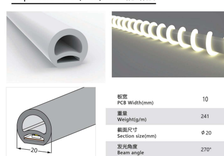
Top View \phi 20 (mm)270° 防断款
