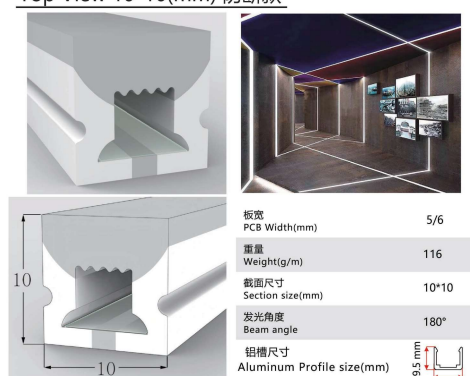
Top View 10*10(mm) 防断款
