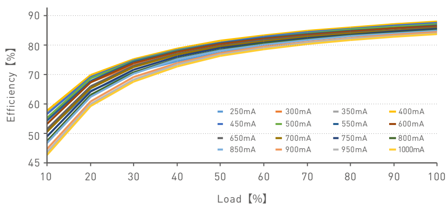
Efficiency vs Load
