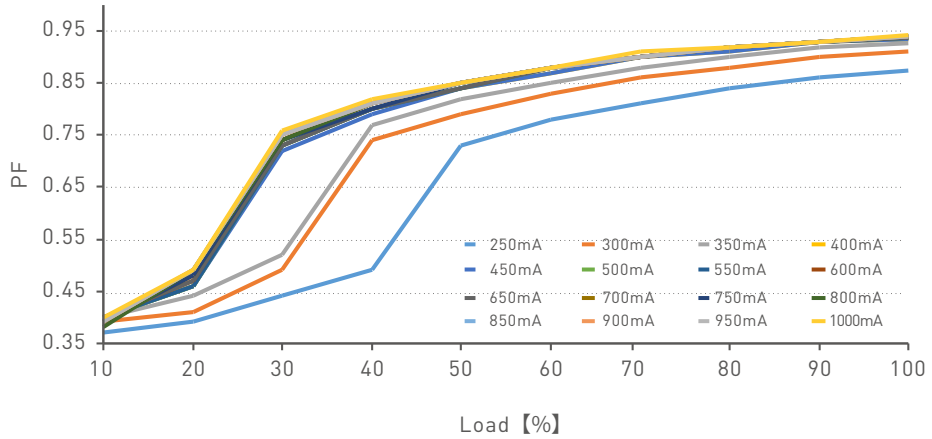
Power Factor Characteristic
