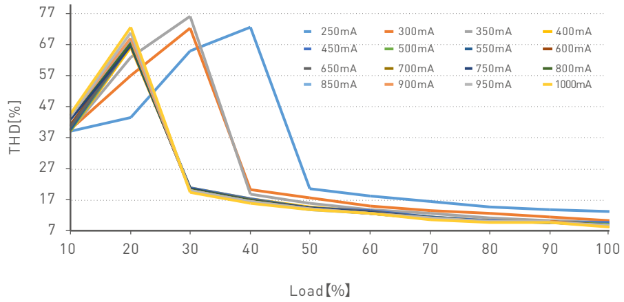
THD vs Load
