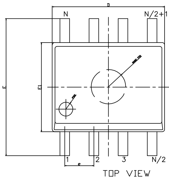
Packaging diagram (ESOP8)
