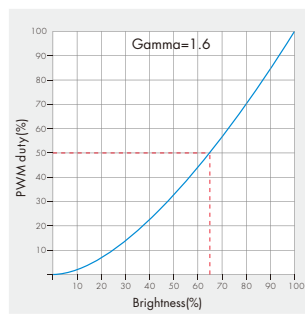
Dimming curve for RGBW/RGB/DIM
