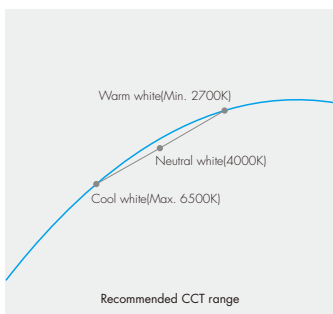
Linear dual color tuning
